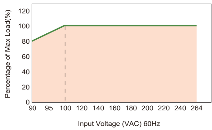
2. Static Characteristics
