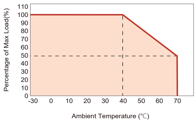
1. Derating Curve
