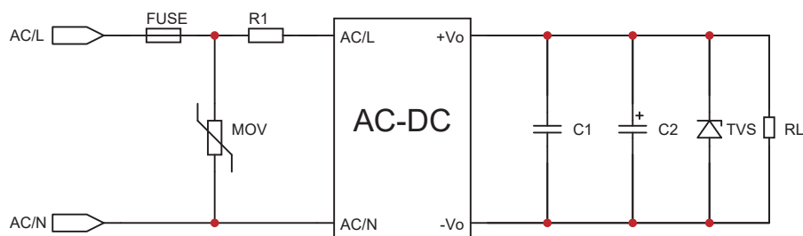
Figure 2: EMC application circuit with higher requirements
