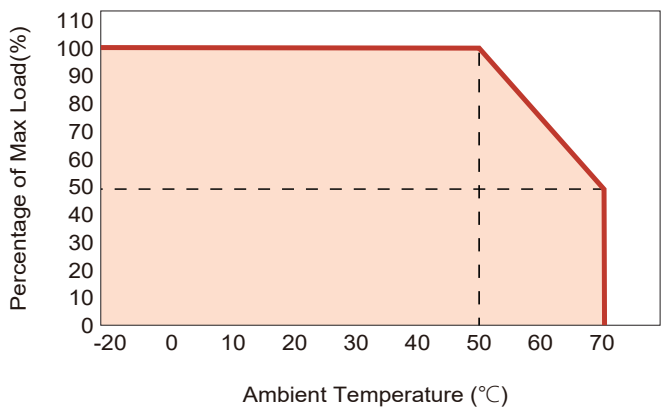
1. Derating Curve
